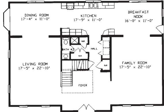
FIRST FLOOR 3744 SQ. FT.
